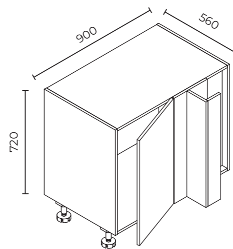
Blind Corner Unit (Reversible) Corner return design flexibility from 50-150mm each-way KI-BA-900-BLIND-CNR
